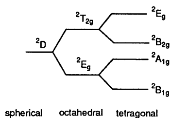
Fig. 4 Energy diagram for copper(II) in spherical, octahedral and tetragonal symmetry fields
