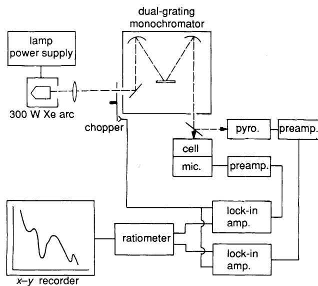
Fig. 1 Block diagram of the photoacoustic spectrometer
