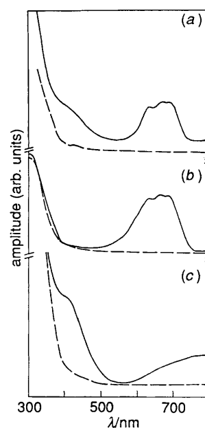
Fig. 2 Photoacoustic spectra of silica gel bonded to N -(2-pyridyl)acetamide. (a) Nickel, (b) cobalt and (c) copper in the visible region. The photoacoustic spectra of silica gel bonded to diacetamide are shown by the broken line.
