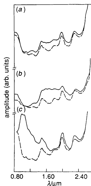
Fig. 3 Photoacoustic spectra of silica gel bonded to N -(2-pyridyl)acetamide. (a) Nickel, (b) cobalt, (c) copper in the near-IR region. The photoacoustic spectra of silica gel bonded to diacetamide are shown by the broken line.
