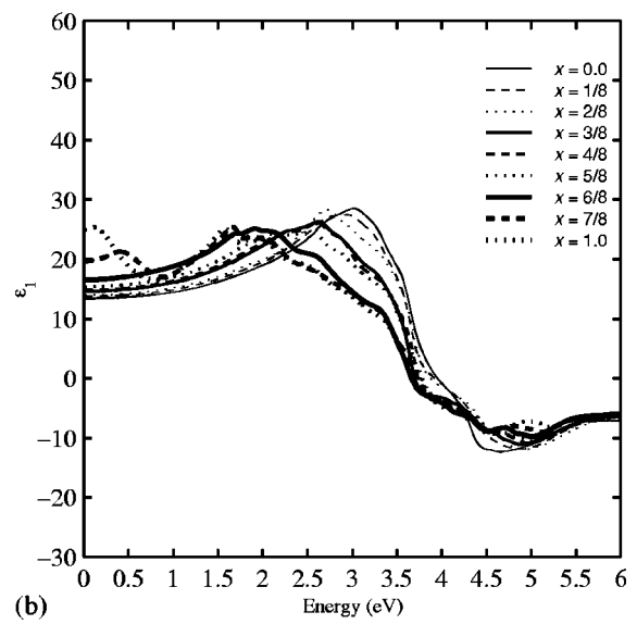
FIG. 4. Measured (a) and calculated (b) real part \epsilon_1(\omega) of the dielectric function.
