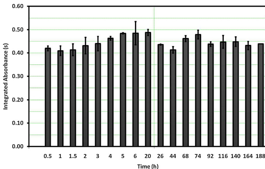
Fig. 4. Influence of the time between the reduction of Se(VI) to Se(IV) and the determination of Se by HG-ET AAS on the integrated absorbance signal; error bars are standard deviation of n=3 repetitive collections and determinations of a 10 \mu\text{g L}^{-1} Se solution.
