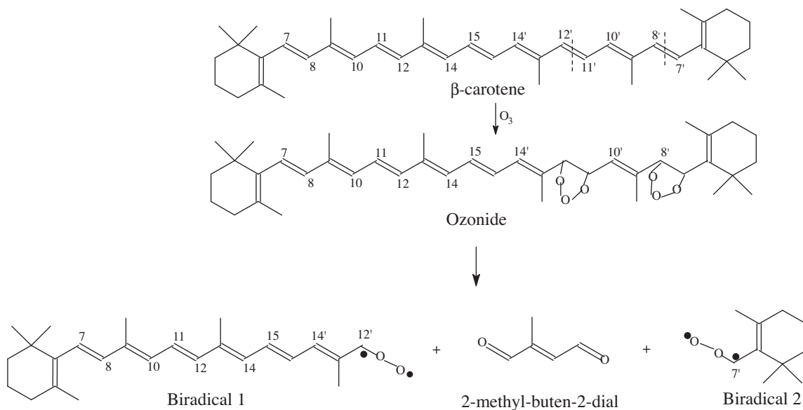
Fig. 2. Proposed mechanism of the formation of 2-methyl-buten-2-dial from the ozonolysis of \beta -carotene.
