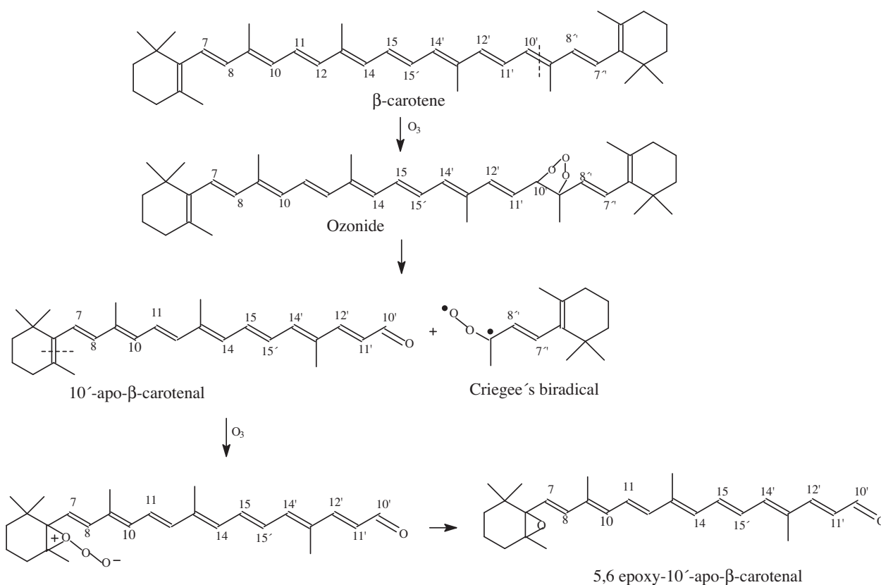
Fig. 3. Proposed mechanism of the formation of epoxycarotenoids (e. g. 5,6-epoxy-10'-apo- \beta -carotenal) from the ozonolysis of \beta -carotene.
