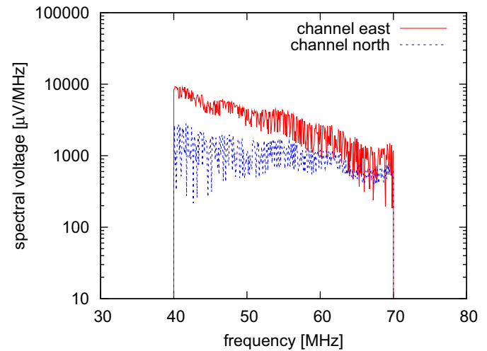
Fig. 8. Time traces (left) and frequency spectra (right) of the simulated event for the east and north channels after folding in the channel response (amplifiers, filters, cable). Note that the cable delays have shifted the time pulses to later times. Also, the spectral bandwidth has been limited to the design bandwidth of the experimental channels, leading to a broadening of the pulses. The signal depicted here is what would be measured at the channel ADCs. Note that the frequency spectra correspond to the complete trace and not the zoomed-in time window shown here.
