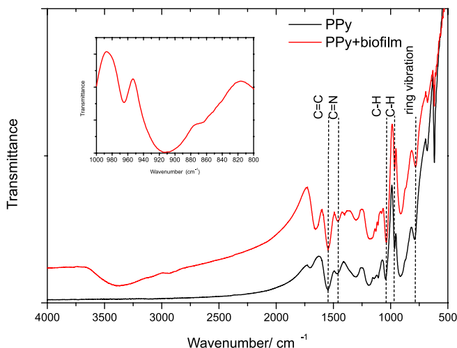
Figure 3. FTIR spectrum of polypyrrole and polypyrrole+ biofilm of S. aureus (in the inset is shown the region around 860 \text{ cm}^{-1} for sample PPy+biofilm)
