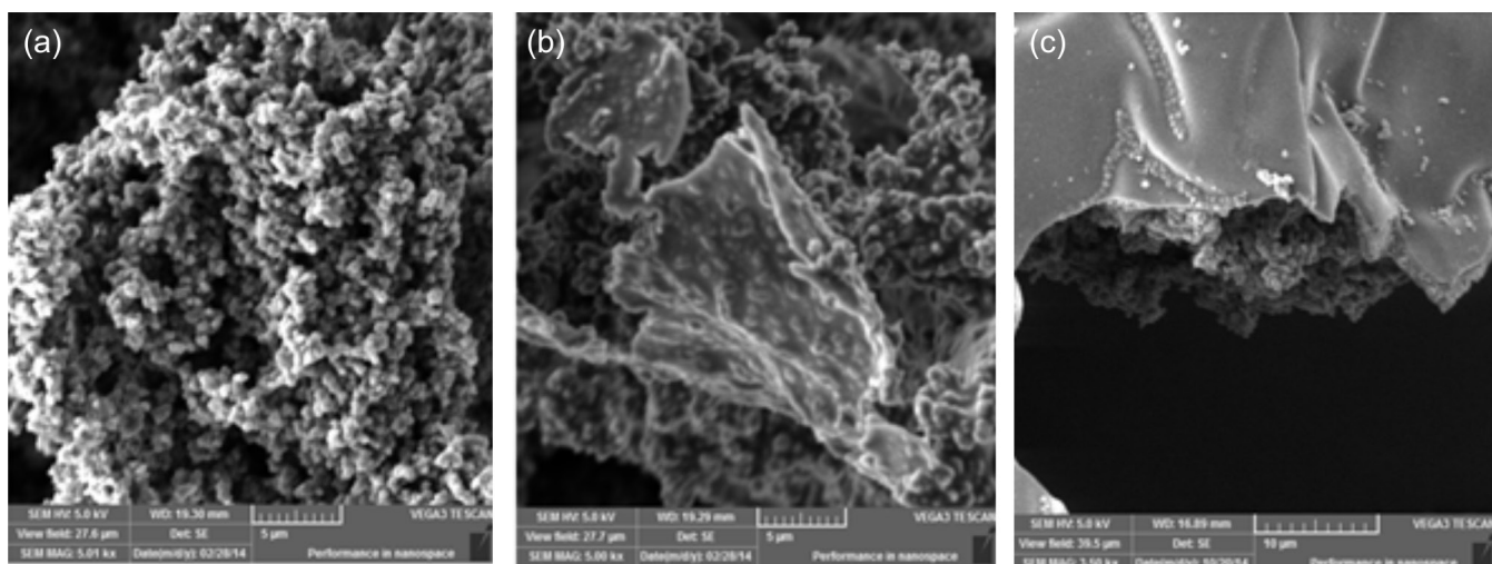
Figure 2. (a) SEM micrograph of as-synthesized polypyrrole, (b) after 6 h and (c) after 120 h of biofilm formation
