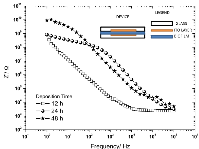
Figure 4. Real part of impedance of biofilms deposited on ITO layers/ glass substrates
