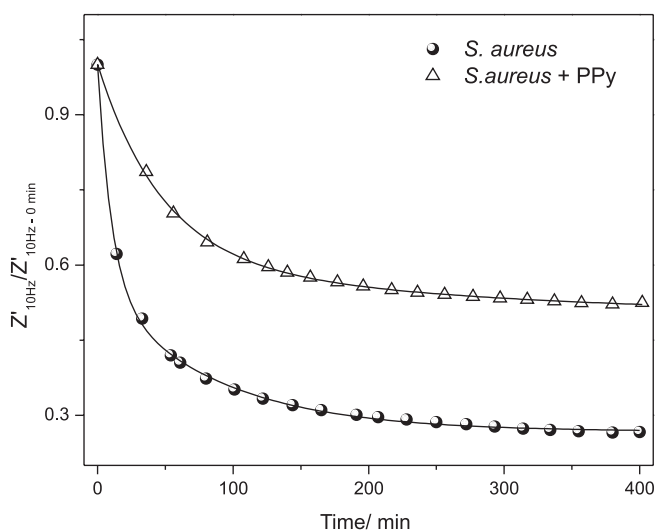
Figure 6. Kinetics of bacterial growth measured by EIS (comparison of polypyrrole-free sample ( S. aureus ) and polypyrrole + S. aureus ( S. aureus +PPy))
