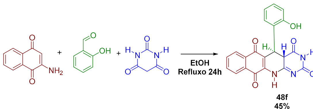
Figura 51: 5-(2-hidroxifenil)-5,12-dihidrobenzo[g]pirimido[4,5-b]quinoline-2,4,6,11(3H,4aH)-tetraona.
