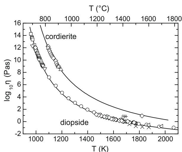
Fig. 1. Viscosity curves of cordierite and diopside liquids. Cordierite: \diamond : this work; \Delta : Giess et al. [35]; \square : Yuritsyn et al. [16]. Diopside: \diamond , \star : this work; \circ : Neville et al. [32]; \square : Sipp et al. [33]; + : Kozu and Kani [30]; \times : McCaffery et al. [31]; \nabla : Taniguchi [34]; \circ : Licko and Danek [29]. Lines: Vogel–Fulcher–Tammann–Hesse (VFTH) fits for cordierite and diopside according to Eqs. (1a) and (1b), respectively.
