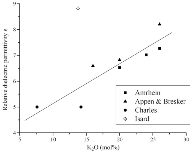
Fig. 4. Experimental relative dielectric permittivity values ( \epsilon ) of \text{K}_2\text{O} - \text{SiO}_2 system [30–33]. Only data from Isard [32] were discarded from analysis.
